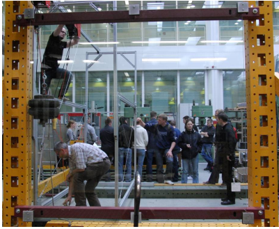
Figure 11: Test set-up.
